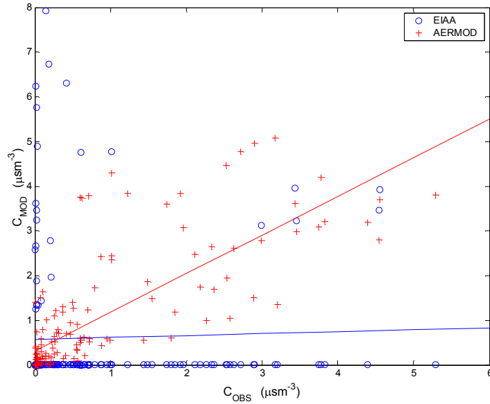
Figure 2 Modeled hourly ground level concentrations (EIAA; AERMOD) versus observed concentrations (normalized by the source strength) of the Alaska tracer field data.
