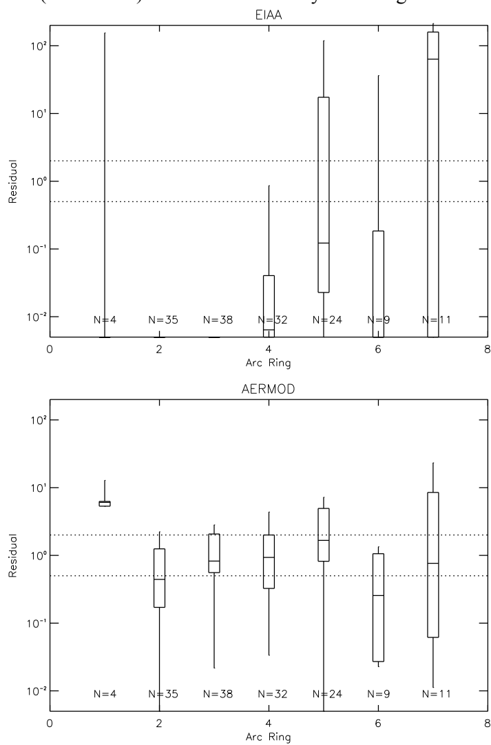
Figure 4 Residual plots of EIAA and AERMOD predictions grouped by arc-ring order. Arc ring order increases with downwind distance from the source (see Table 2).
