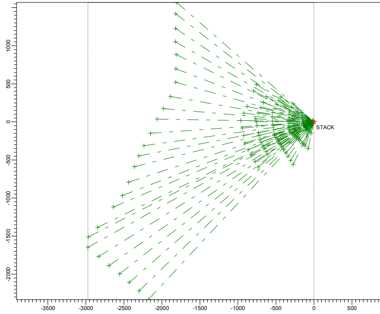
Figure 1 AERMOD computation domain and discrete receptors.
