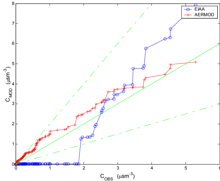
Figure 3 Quantile-quantile plots of modeled hourly ground level concentrations (EIAA; AERMOD) versus observed concentrations (normalized by source strength) of the Alaska tracer field data.
