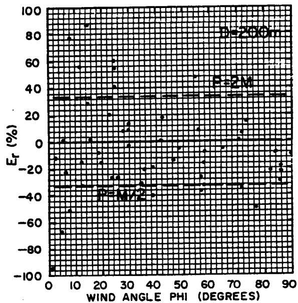
RELATIVE ERROR, E_r , VERSUS WIND ANGLE FOR GROUND-LEVEL RECEPTORS ( Z=0.5m )—CALTRANS HIGHWAY 99 TRACER STUDY
