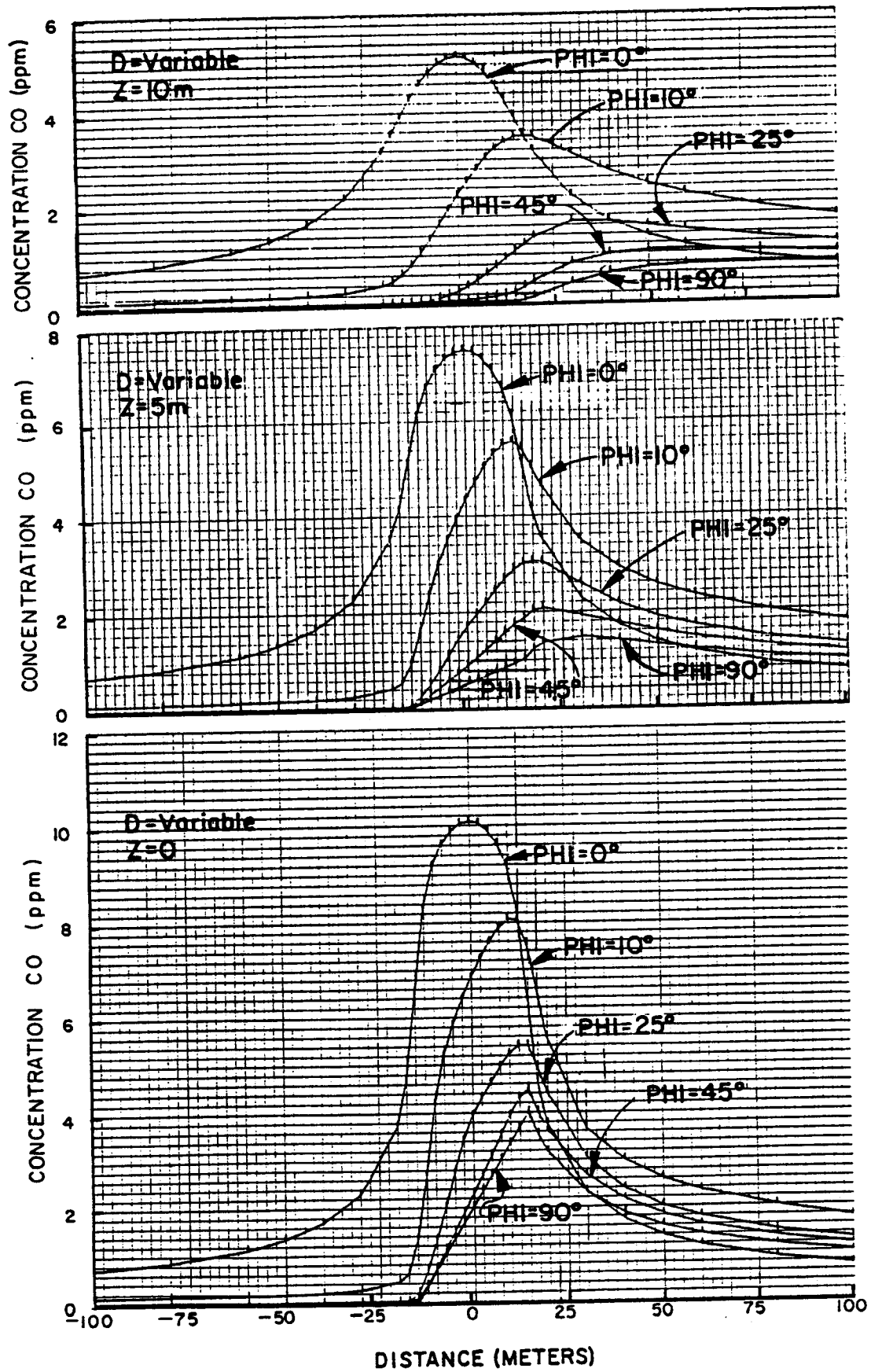
CALINE4 SENSITIVITY ANALYSIS— VARIABLE: WIND ANGLE (PHI)
