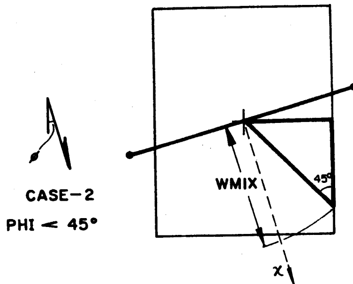
ELEMENT GEOMETRY FOR DETERMINING WMIX
