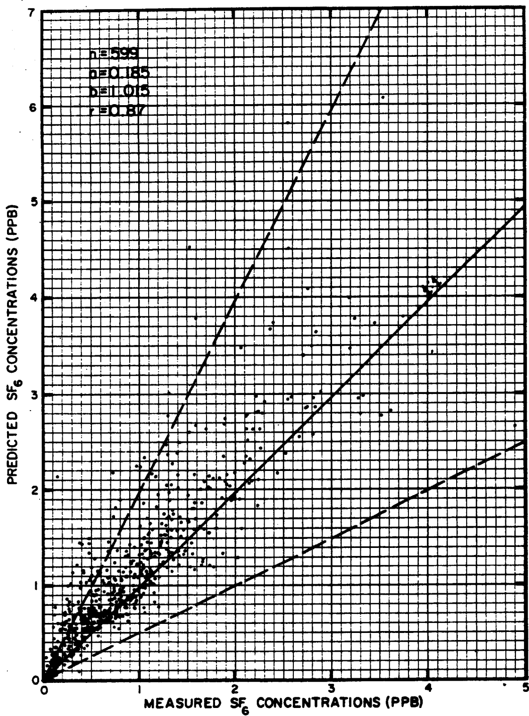
CALINE4 SCATTERPLOT FOR GENERAL MOTORS DATA FIGURE 46
