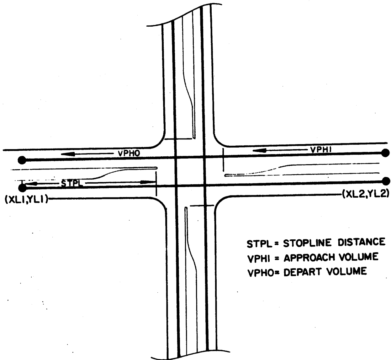
CALINE4 INTERSECTION LINKS
