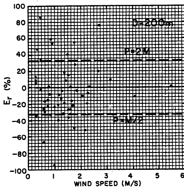
RELATIVE ERROR, E_r VERSUS WIND SPEED FOR GROUND LEVEL RECEPTORS ( Z=1.0m )—CALTRANS HIGHWAY 99 TRACER STUDY
