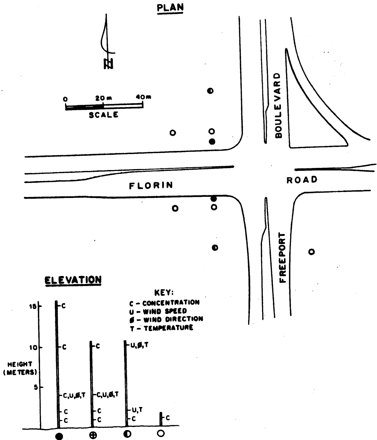
CALTRANS SACRAMENTO (SACTO) INTERSECTION TEST SITE
