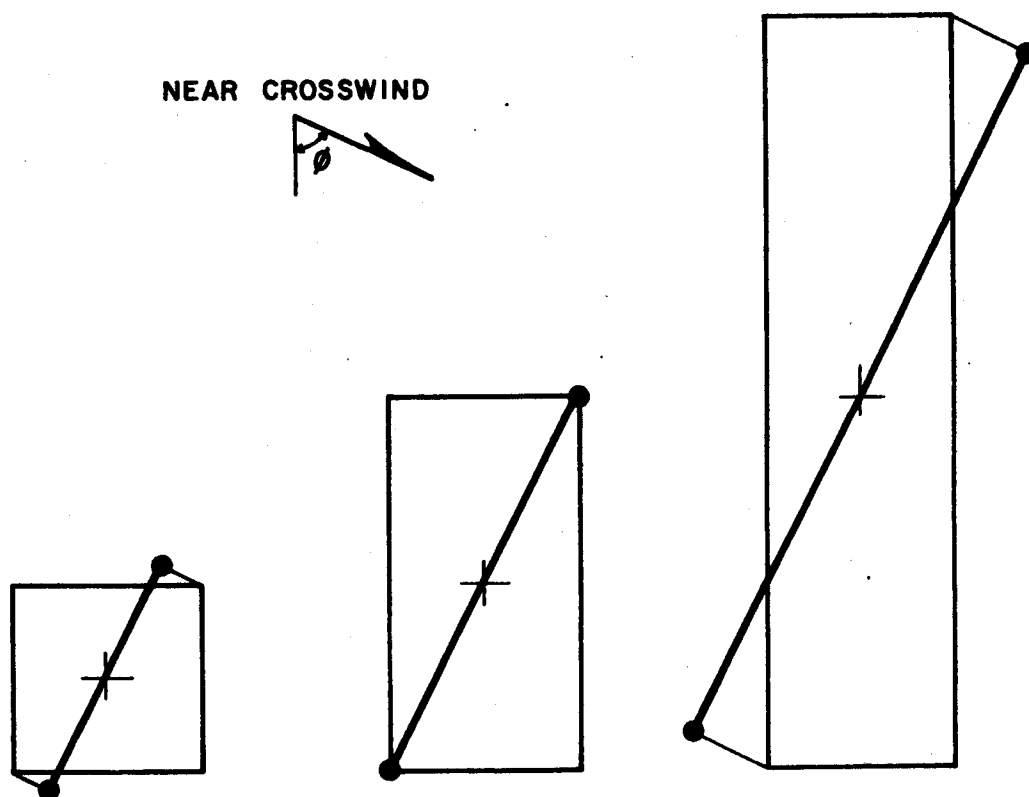
EQUIVALENT FINITE LINE SOURCE REPRESENTATION FOR VARIOUS ELEMENT SIZES AND WIND ANGLES
