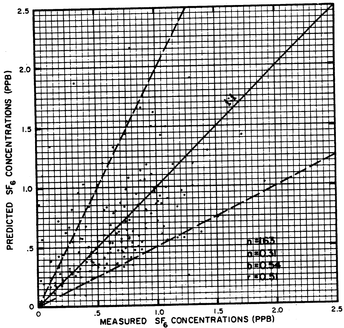
CALINE4 SCATTERPLOT FOR CALTRANS HIGHWAY 99 TRACER STUDY
