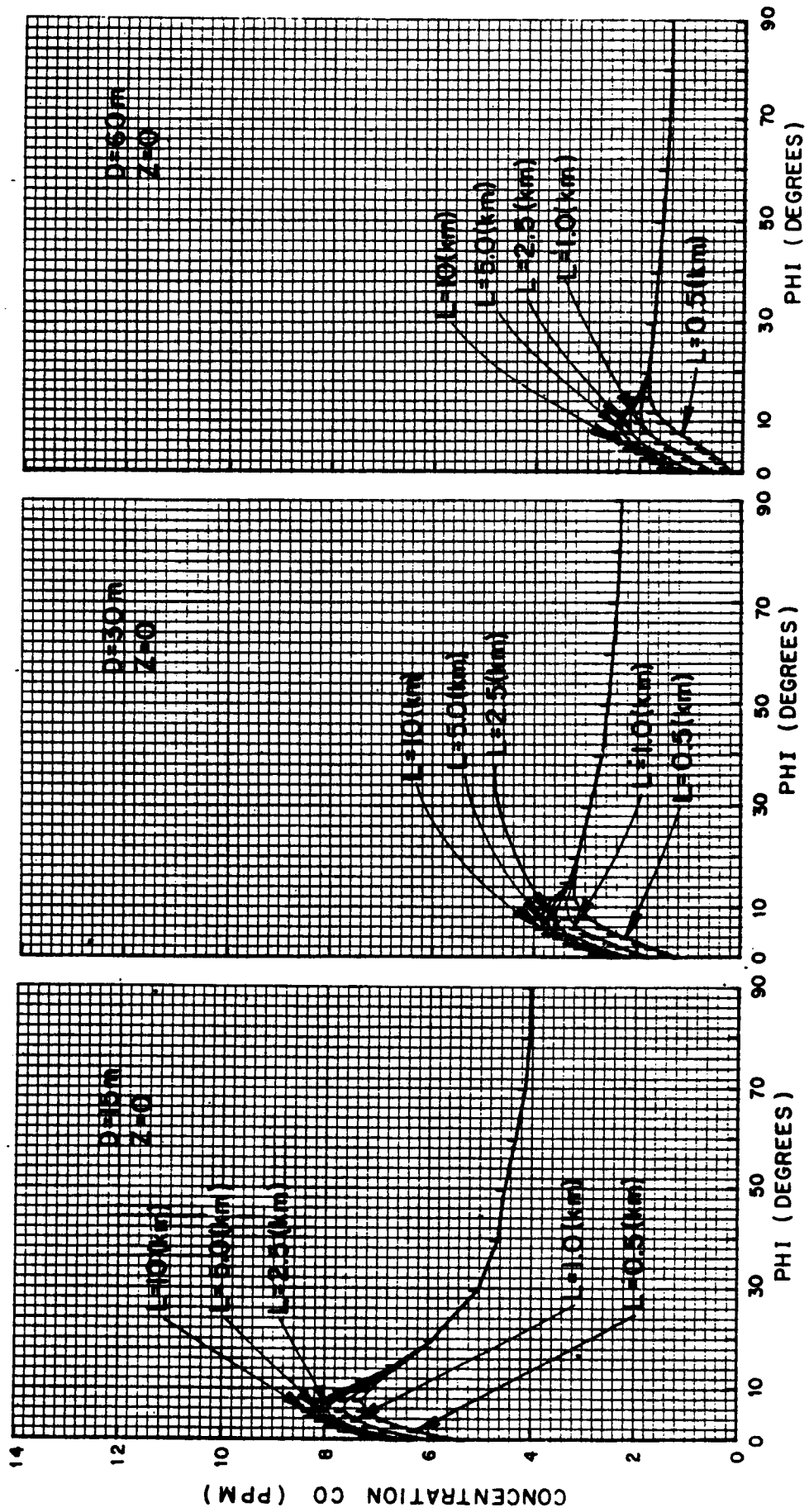
CALINE4 SENSITIVITY ANALYSIS—VARIABLE: HIGHWAY LENGTH (L) FIGURE 31
