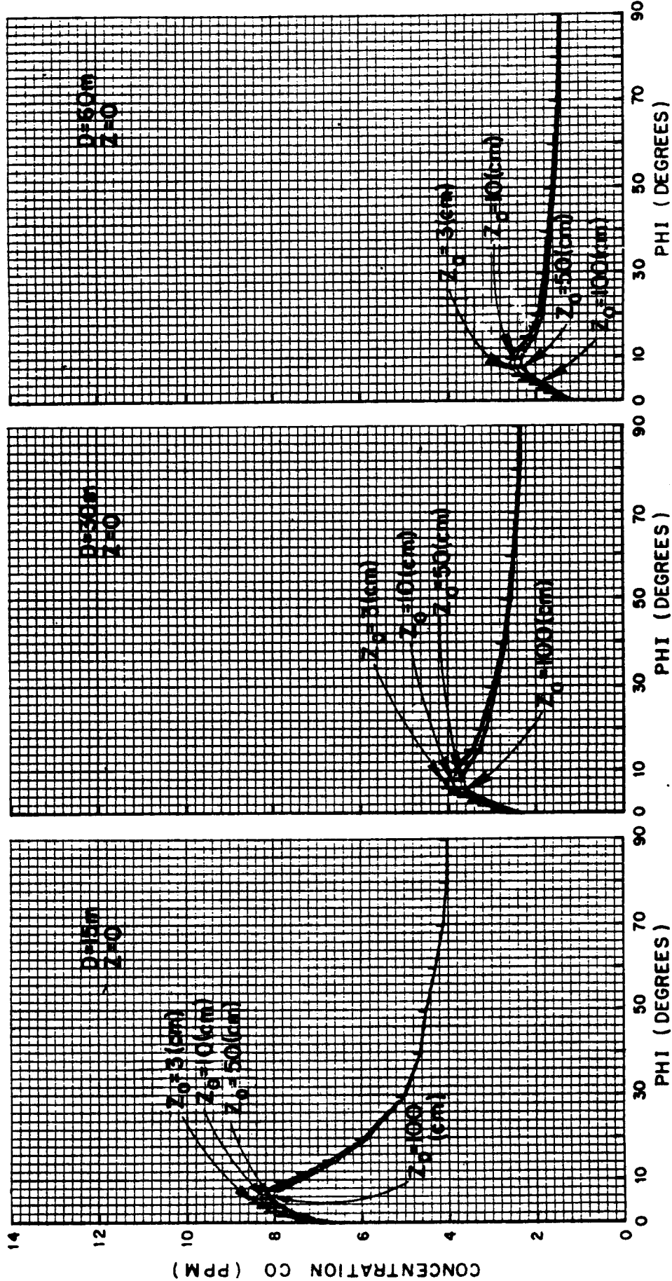
CALINE4 SENSITIVITY ANALYSIS — VARIABLE: ROUGHNESS (Z 0 )
