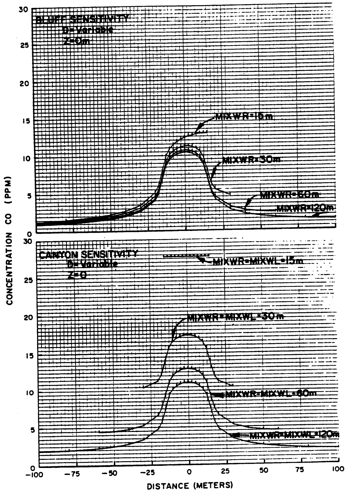
CALINE4 SENSITIVITY ANALYSIS—VARIABLE: MIXING WIDTH (MIXWR, MIXWL)
